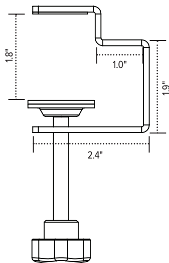
mounting bracket
