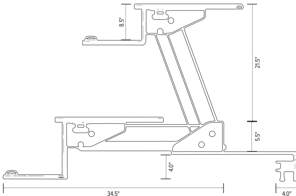
Lift Side view
