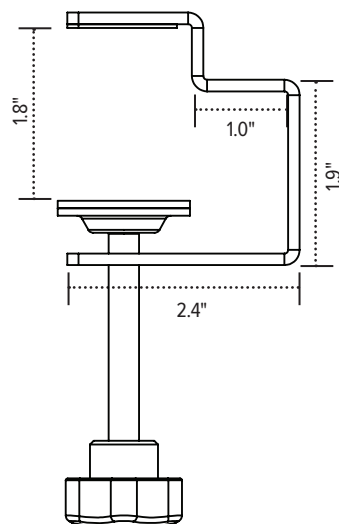
mounting bracket
