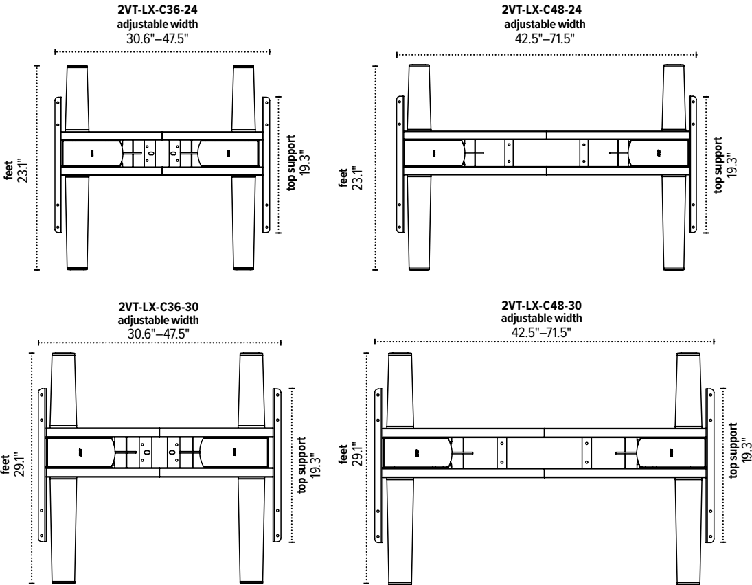
The base dimensions as shown are actual.
