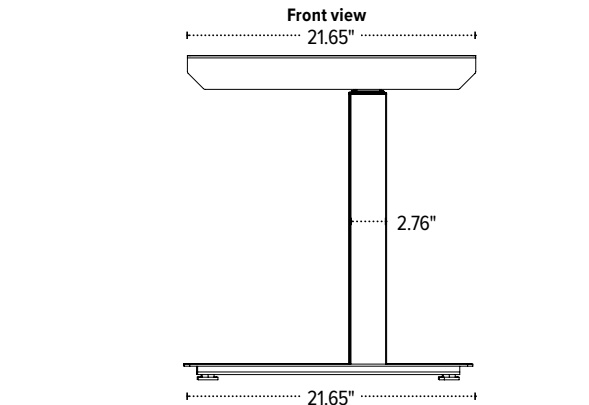
The base dimensions as shown are actual.
