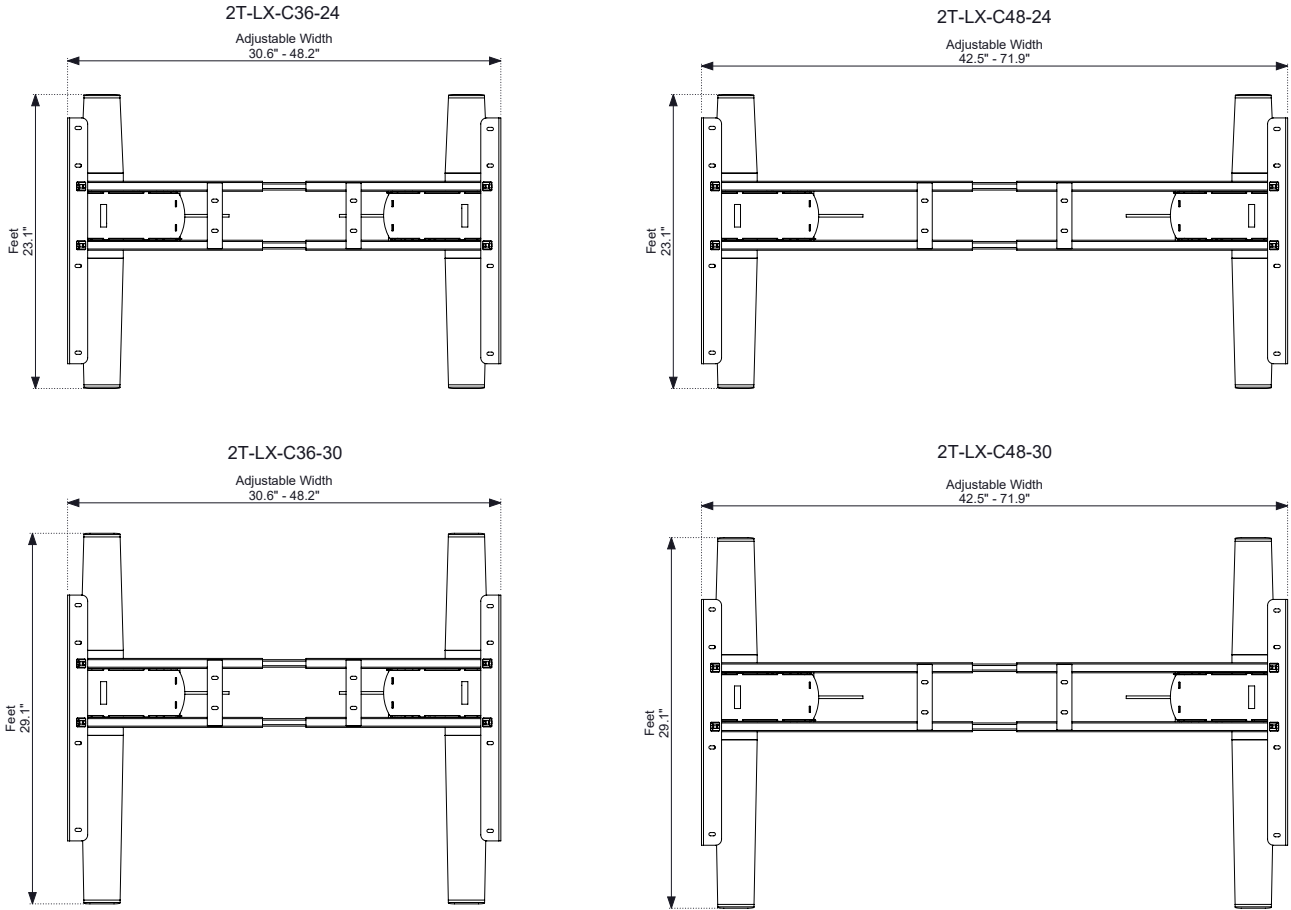
The base dimensions as shown are actual.
