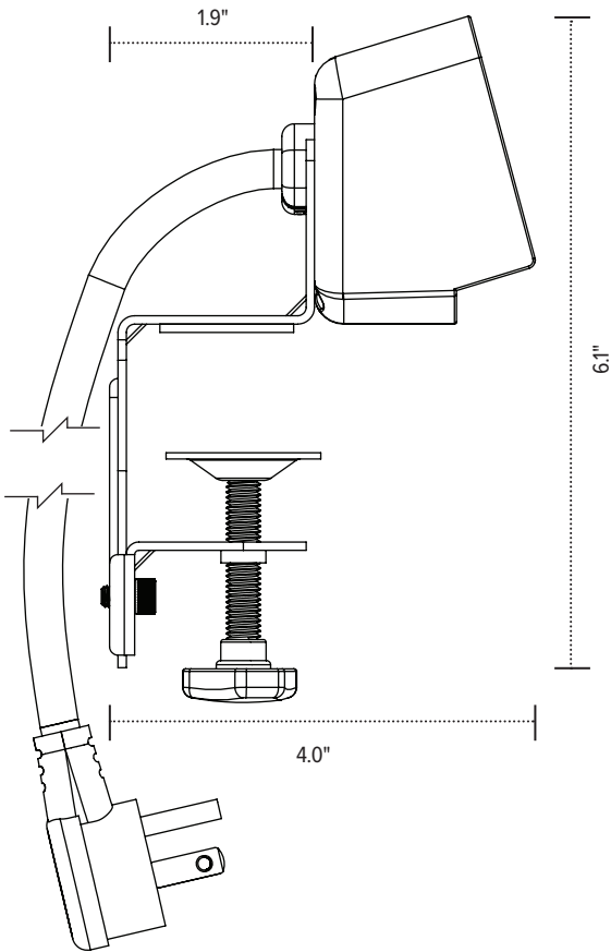
Side view
