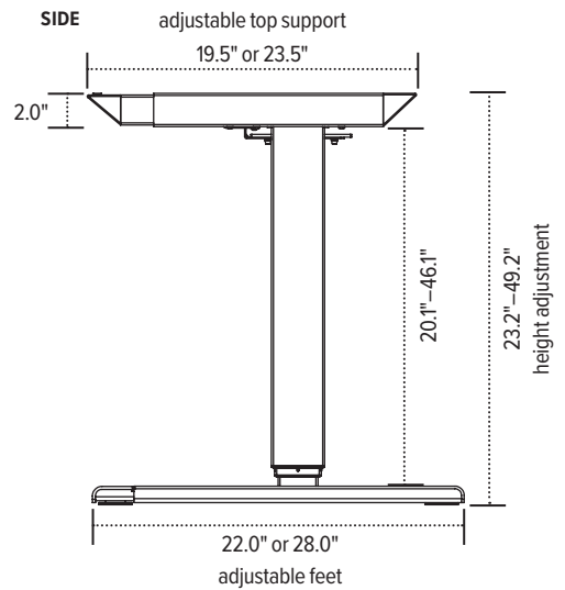
SIDE
