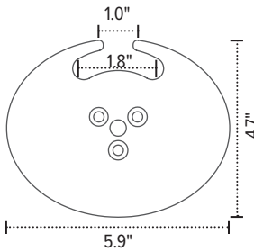
Bottom grommet mount plate
