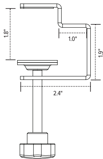
mounting bracket
