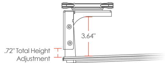
SIDE VIEW HEIGHT EXPANDED
