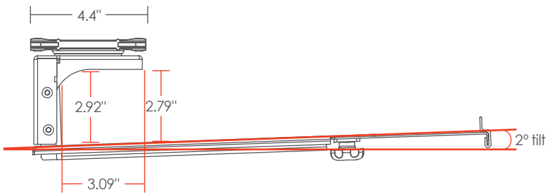
SIDE VIEW HEIGHT RETRACTED
