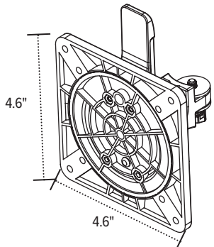
VESA plate
