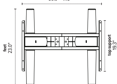
2VT-LX-C36-24 adjustable width 30.6"–47.5"
