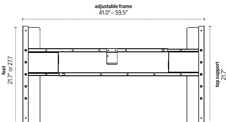
2TC-C48-24-___ Top view
