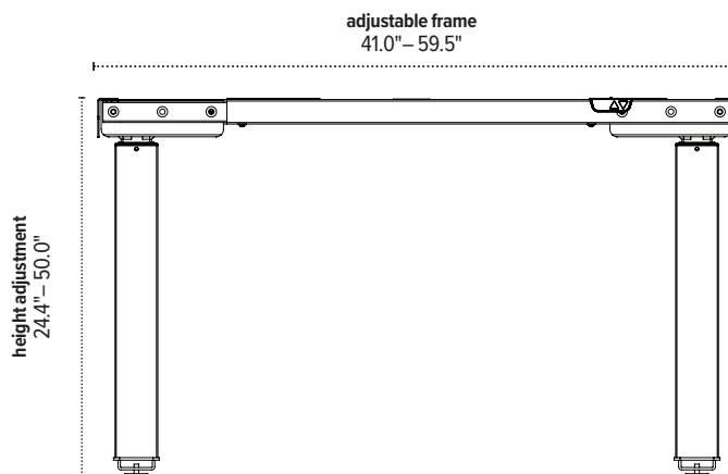
2TC-C48-24-___ Front view
